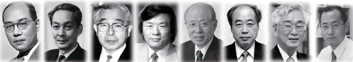
Hideki Yukawa 1949
